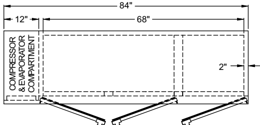
Plan View
